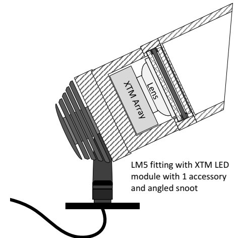
LM5 fitting with XTM LED module and 2 accessories
