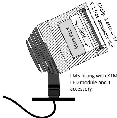
LM5 fitting with XTM LED module and no accessories.
