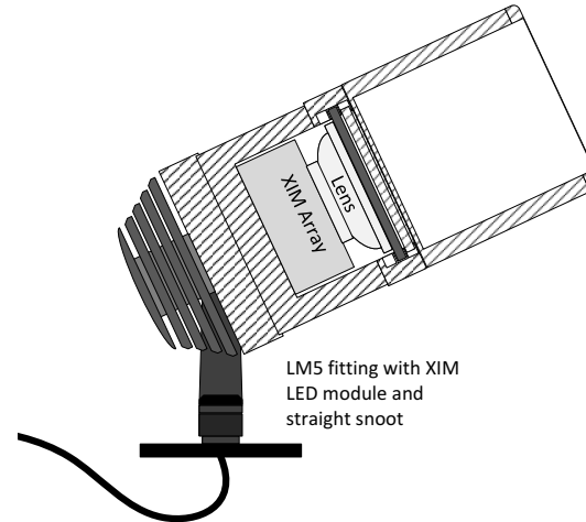
LM5 fitting with XIM LED module and either honeycomb or diffuser
