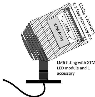
LM6 fitting with XTM LED module and no accessories.
