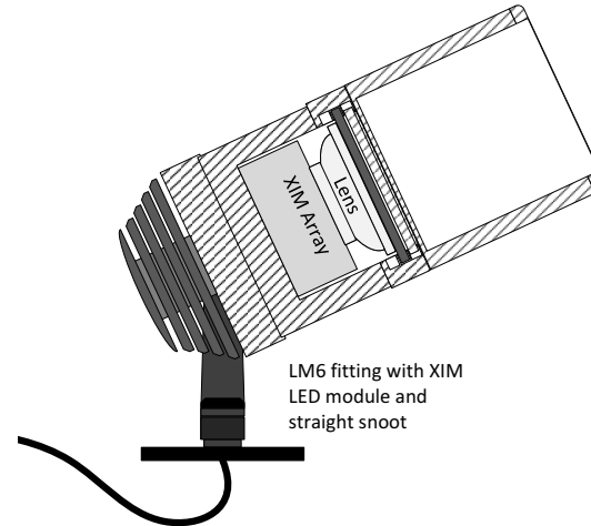
LM6 fitting with XIM LED module and either honeycomb or diffuser
