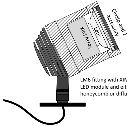
LM6 fitting with XIM LED module and no accessories.
