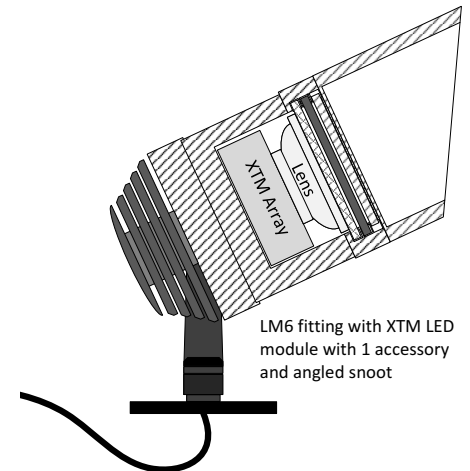
LM6 fitting with XTM LED module and 2 accessories
